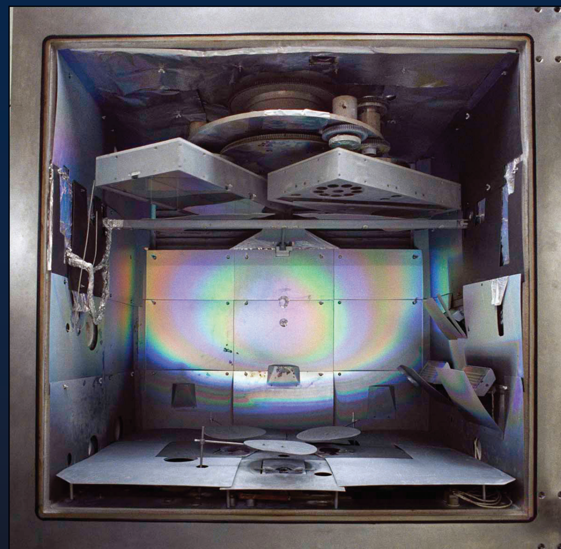
OMAN's large coater with a NIF polarizer
